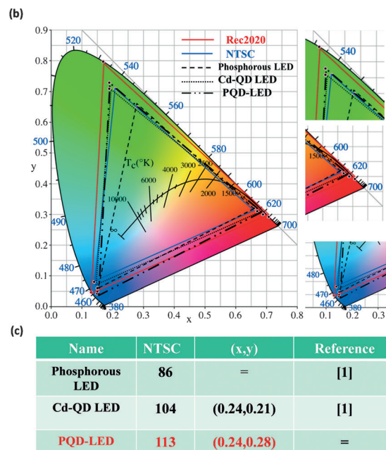
Figure 9. a) Spectra of PQD-based white LED before color filter, b) color gamut of PQD-LED, phosphor LED, and Cd-QDs white LED c) The table features data of the three types of display.
