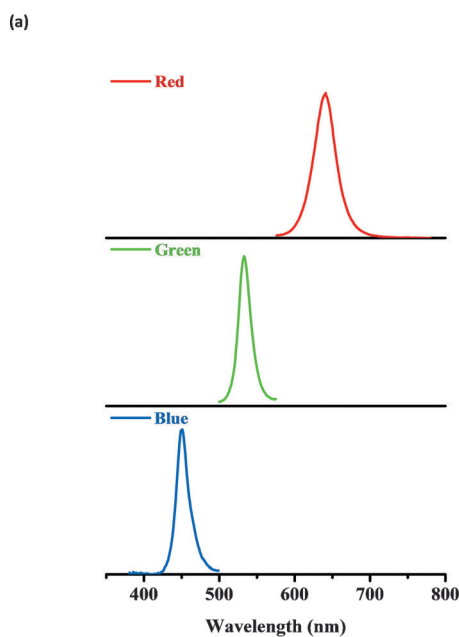
Figure 9. a) Spectra of PQD-based white LED before color filter, b) color gamut of PQD-LED, phosphor LED, and Cd-QDs white LED c) The table features data of the three types of display.
